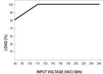
■ Static characteristic
