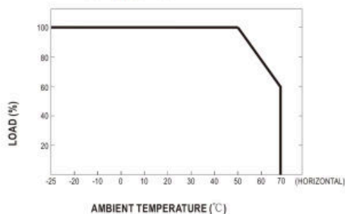
■ Derating Curve
