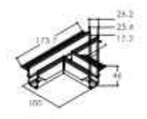
MG-321-20-AT Size: 173.5*100*46mm Material: Aluminum
