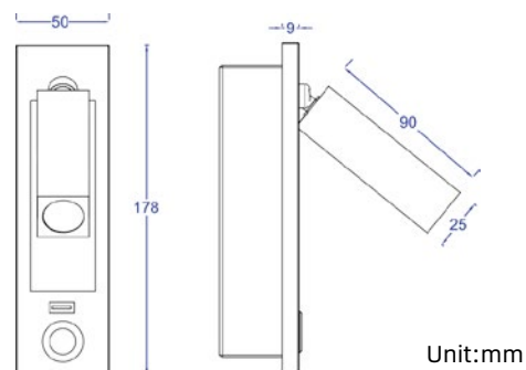
Cutout size: L160 x W40 x H60mm
