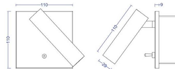
Cutout size: L95 x W60 x H40mm
